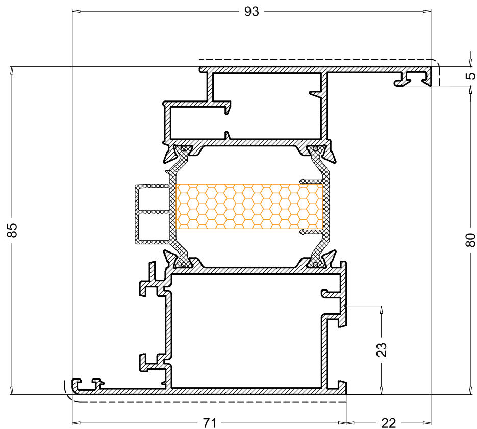
PE85214 2.046 Kg/m
