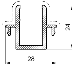
PS15008 0.394 Kg/m
