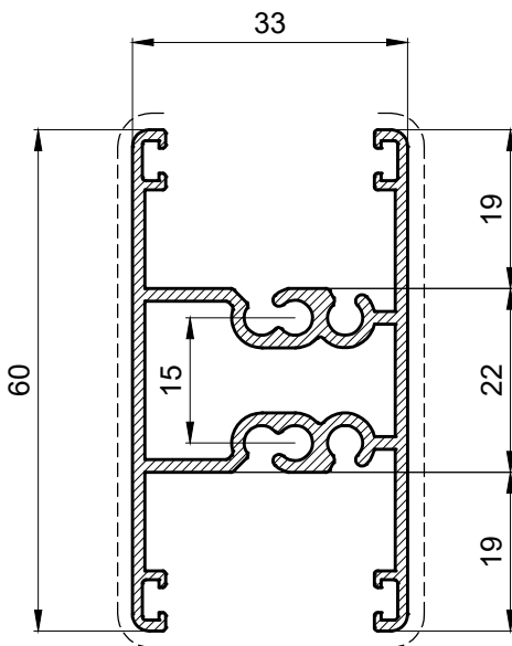
PS15062 0.954 Kg/m
