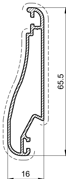
PS15004 0.484 Kg/m
