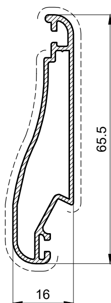
PS15004 0.484 Kg/m
