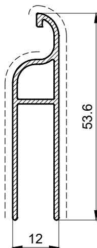
PS15003 0.382 Kg/m
