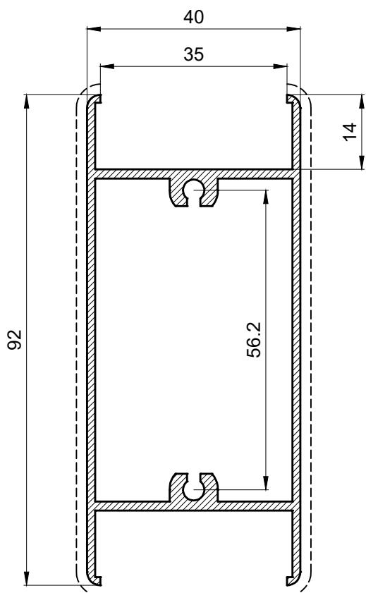
PM 40047 1,246 Kg/m
