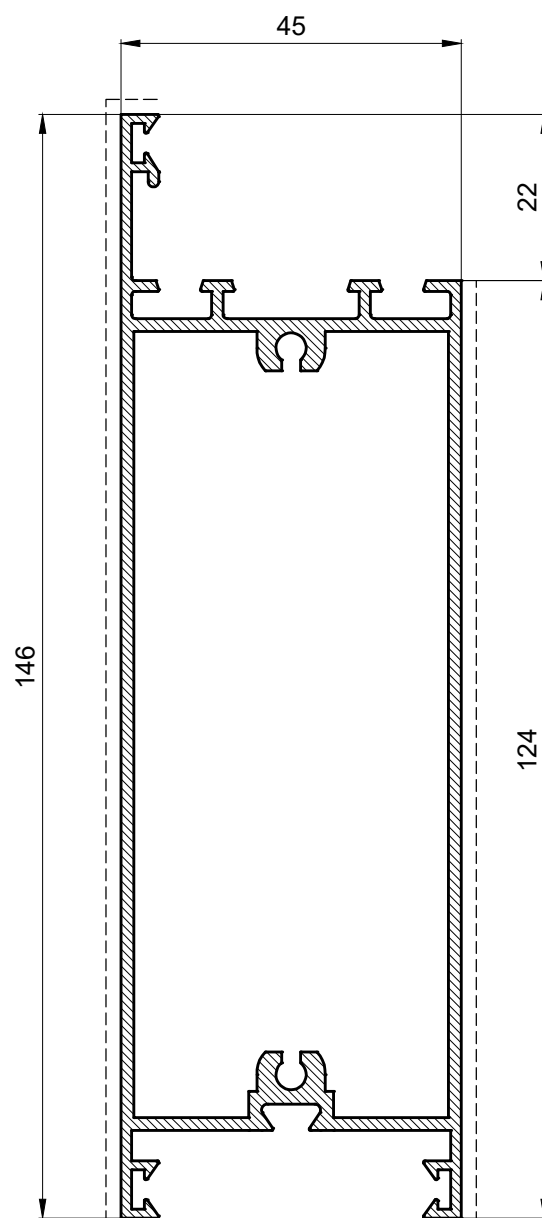
PM 40022 1,955 Kg/m
