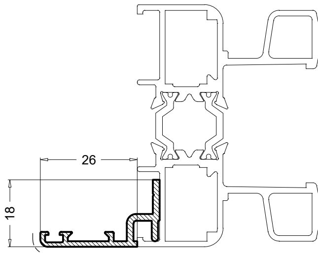
PS15601 0.269 Kg/m
